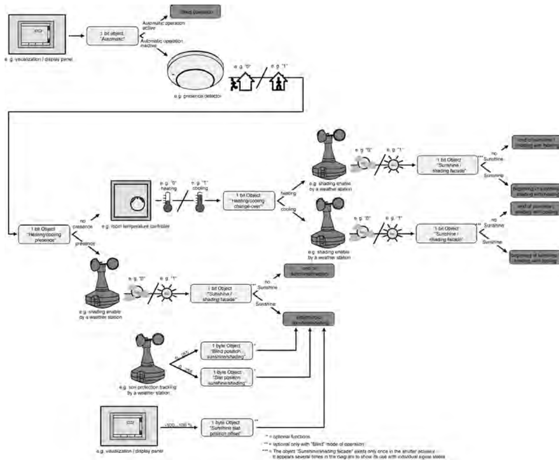
picture 30: Schematic diagram of automatic heating/cooling (for reasons of simplicity shown without disabling functions of the automatic or direct operation)
