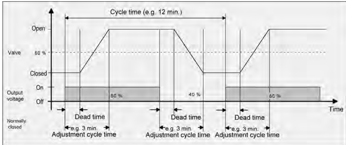
picture 46: Ideal course of the valve stroke for a command value of approx. 60 % of a deenergised, closed valve
