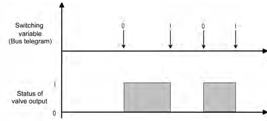
picture 35: Conversion of a switching command value to an output signal with deenergised, opened valve drives (example)
