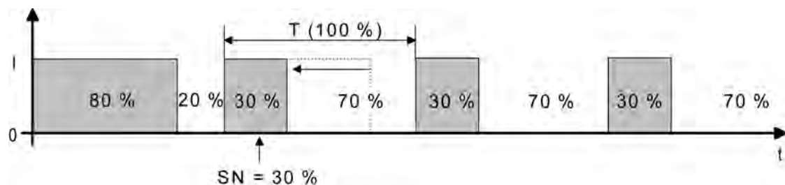
picture 40: Command value change, e.g. from 80 % to 30 % during the opening phase of the valve
