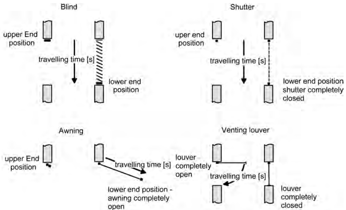
picture 11: Determining the movement time according to the drive type
