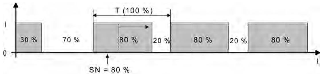
picture 43: Command value change, e.g. from 30 % to 80 % during the opening phase of the valve
