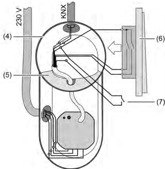
picture 3: Installing the device in an electronics box (example)
