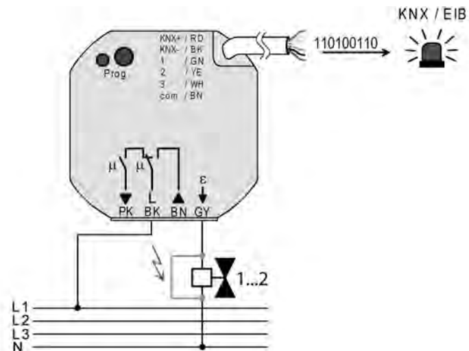
picture 49: Short-circuit and overload detection in case of fault in valve output or valve drive
