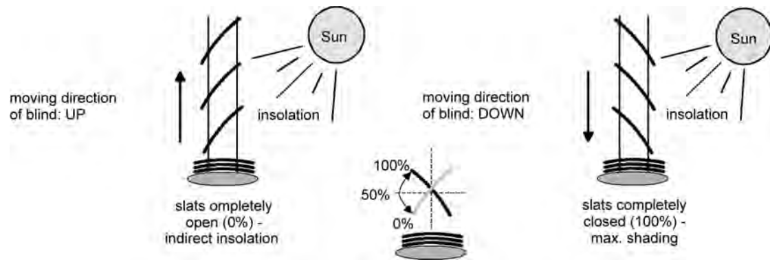
picture 12: Type 1 - Slatted Venetian blinds with oblique slat position in both travel directions
