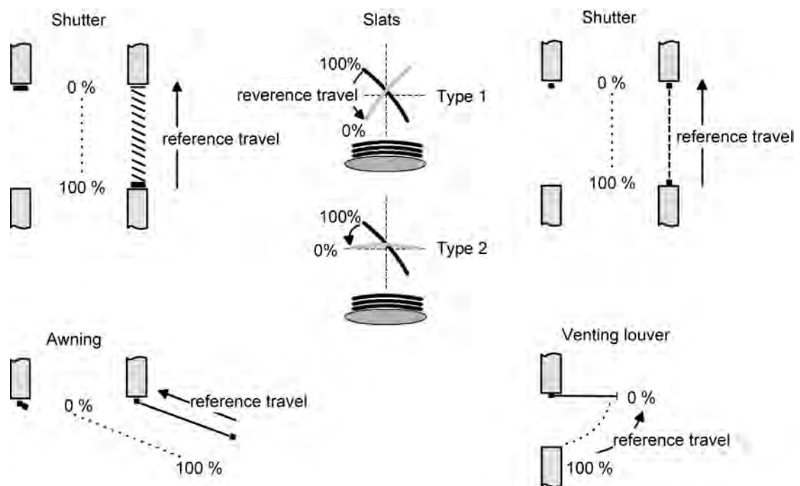
picture 17: Reference movement
