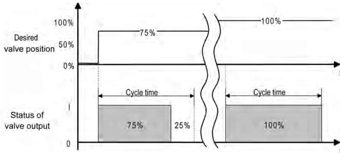
picture 34: Conversion of a constant valve setpoint position to an output signal with deenergised, closed valve drives (example)
