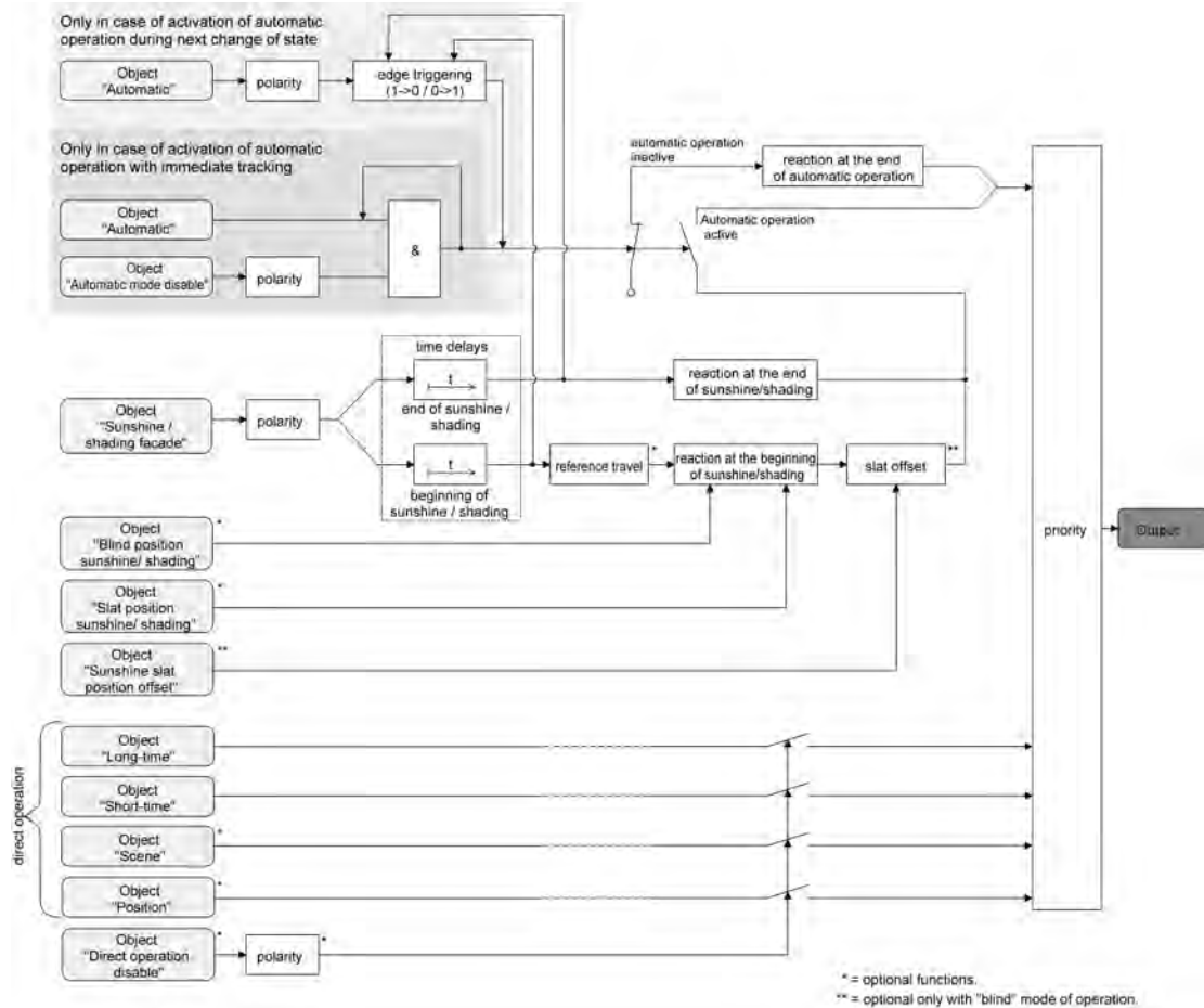
picture 23: Function diagram illustrating the extended sun protection
