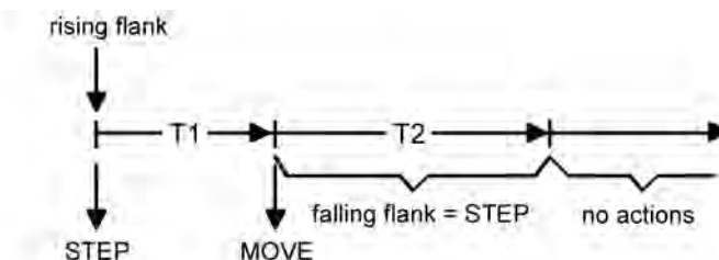
picture 7: Operation concept "short – long – short"
