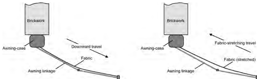
picture 32: Fabric stretching in an awning
