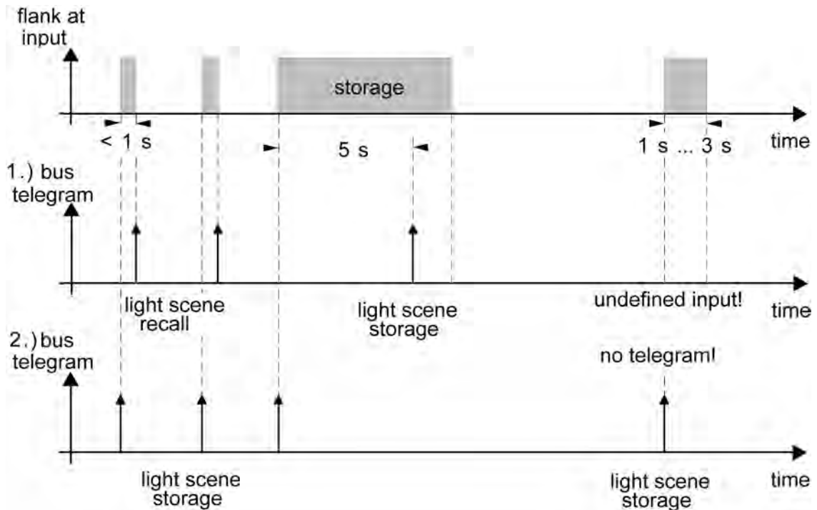
picture 10: Example of scene storage
