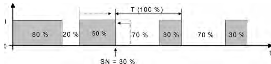
picture 42: Command value change, e.g. from 80 % to 30 % during the opening phase of the valve (opening phase too long)
