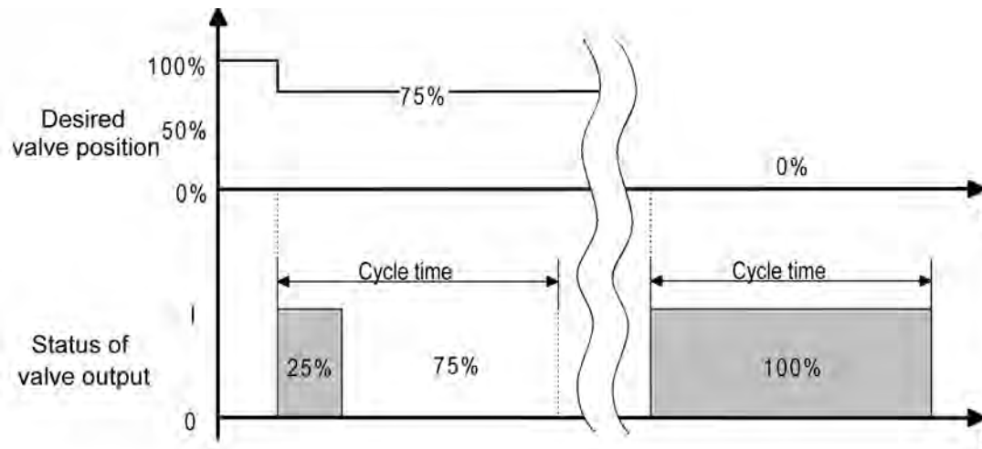
picture 36: Conversion of a constant valve setpoint position to an output signal with deenergised, opened valve drives (example)
