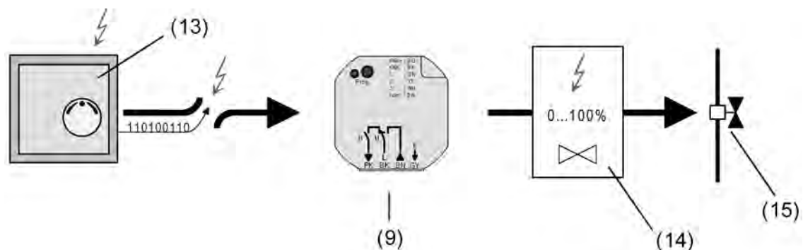
picture 48: Principle of cyclical command value monitoring in the event of a fault (e.g. open circuit)
