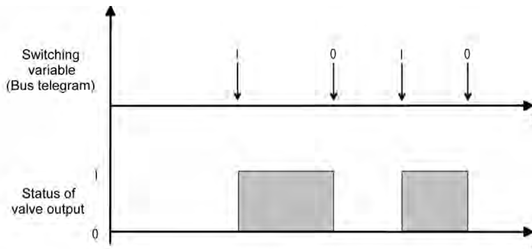
picture 33: Conversion of a switching command value to an output signal with deenergised, closed valve drives (example)
