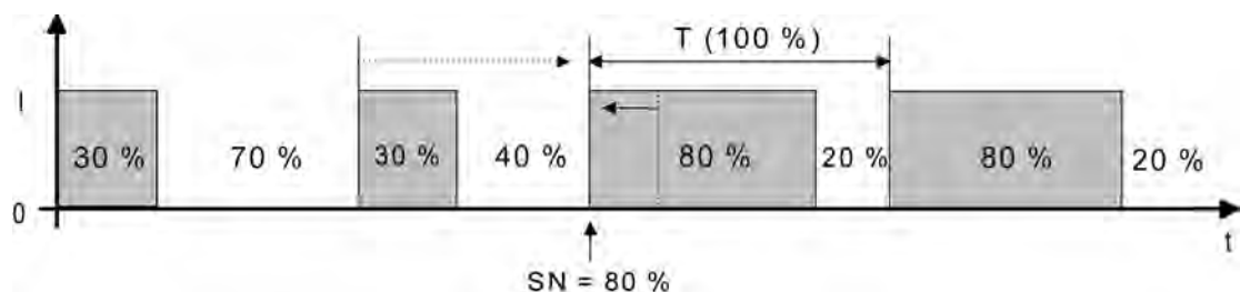
picture 45: Command value change, e.g. from 30 % to 80 % during the closing phase of the valve (closing phase too long)
