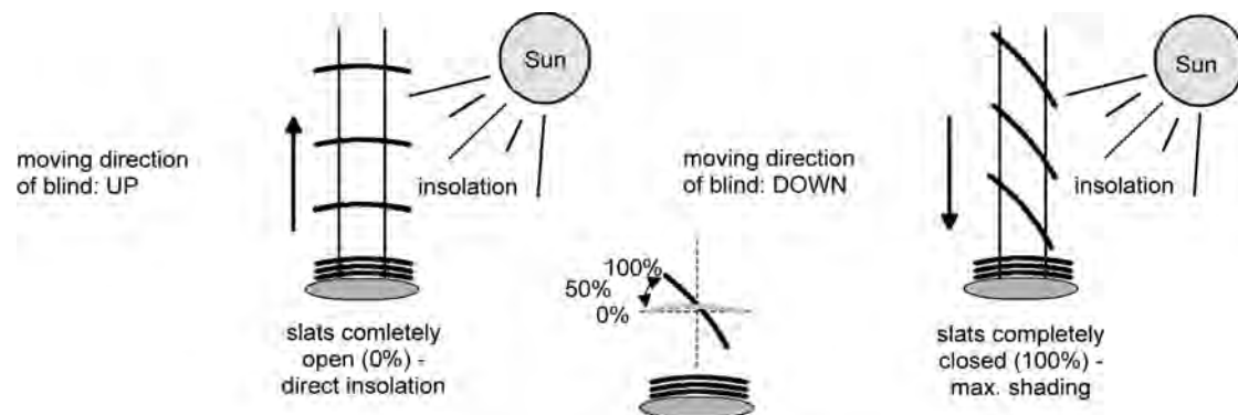
picture 13: Type 2 - Slatted Venetian blinds with oblique and horizontal slat position
