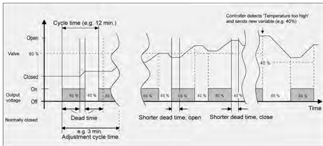
picture 47: Ideal course of the valve stroke for a command value of approx. 60 % at first of a deenergised, closed valve
