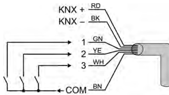
picture 5: Connection of the extension inputs
