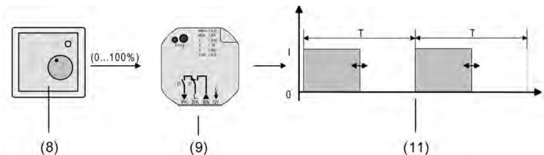
picture 38: Command value principle for constant command value
