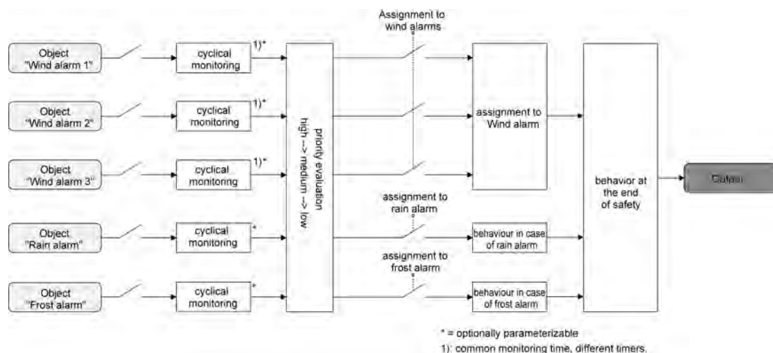
picture 18: Function diagram of the safety function
