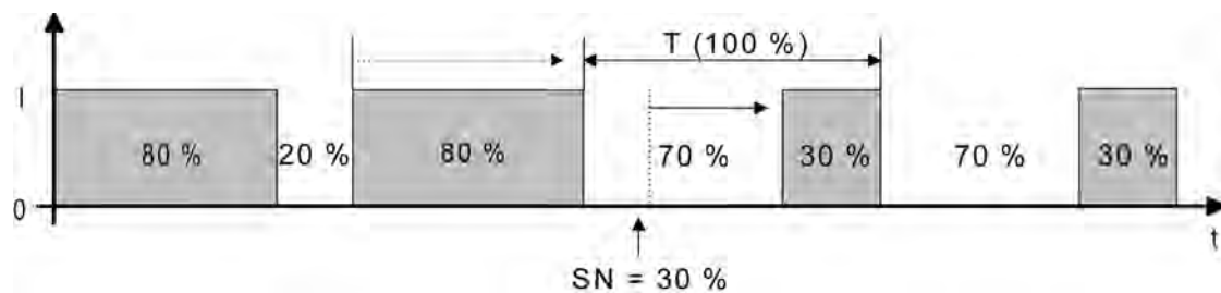
picture 41: Command value change, e.g. from 80 % to 30 % during the closing phase of the valve
