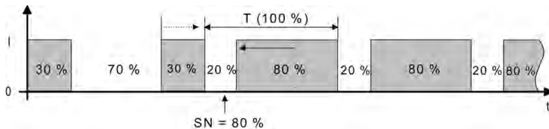
picture 44: Command value change, e.g. from 30 % to 80 % during the closing phase of the valve
