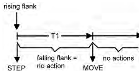
picture 8: Operation concept "long – short"
