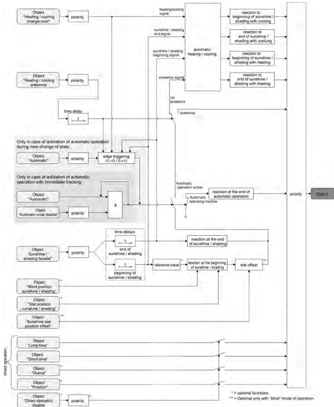
picture 31: Schematic function diagram of automatic heating/cooling
