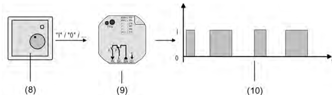
picture 37: Command value principle for switching command value
