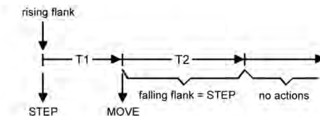
picture 6: Operating concept "Short - long - short" when inputs 1 and 2 have an internal impact
