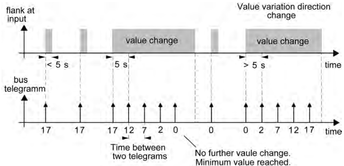
picture 9: Example to change the value for dimming value encoder
