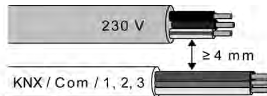
picture 2: Minimum cable spacing
