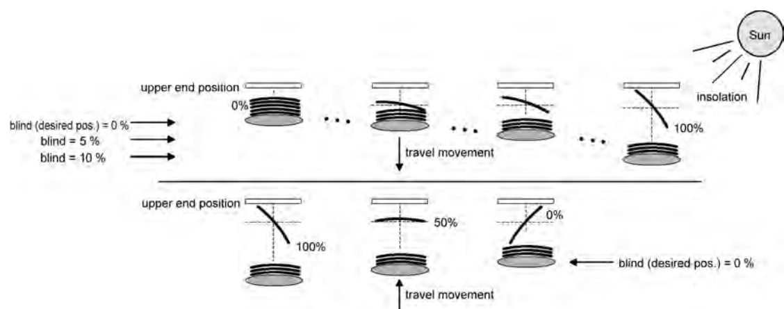
Figure 16: Example of slat positioning with the Venetian blind in upper end position (typical of slat type 1)
