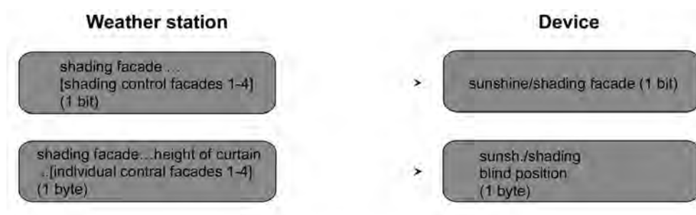
Figure 29: Programming of the communication objects for application example V
