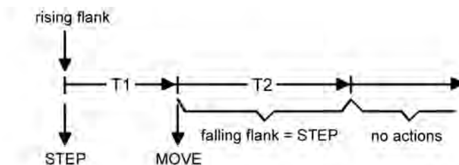
Figure 6: Operating concept "Short - long - short" when inputs 1 and 2 have an internal impact
