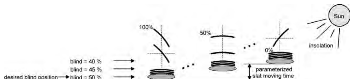
Figure 15: Example of slat positioning affecting the position of the Venetian blind (typical of slat type 1; analogous reaction for type 2)
