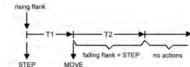
Figure 7: Operation concept "short – long – short"
