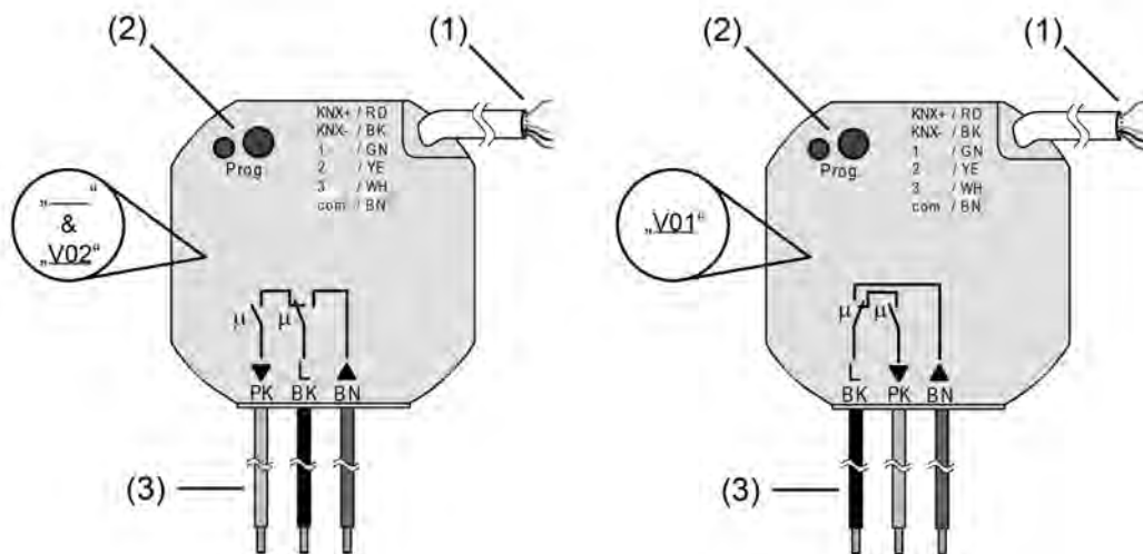
Figure 1: Device components
