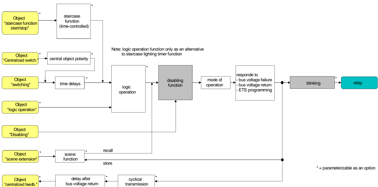
Fig. 19: Functional diagram of the disabling function
