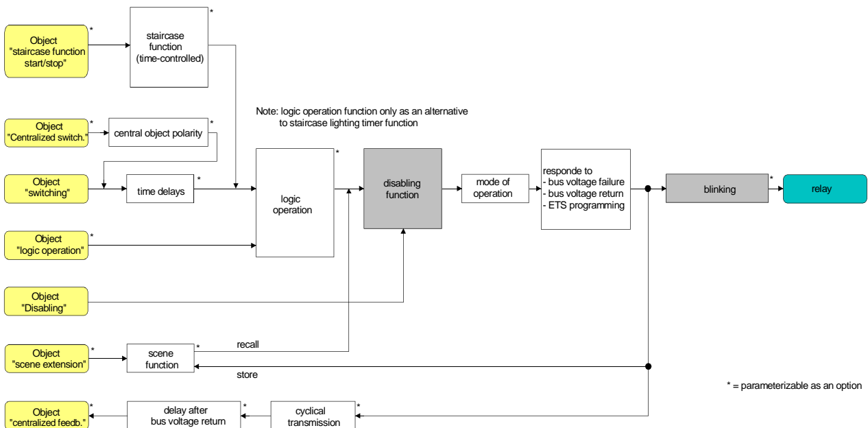
Fig. 17: Functional diagram of the disabling function
