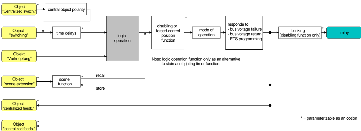
Fig. 19: Functional diagram of the logic function
