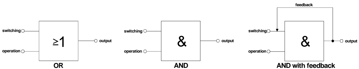
Fig. 20: Gating operations of the logic function
