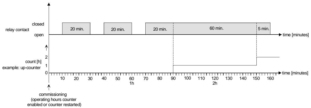
Fig. 16: Functional principle of the operating hours counter
