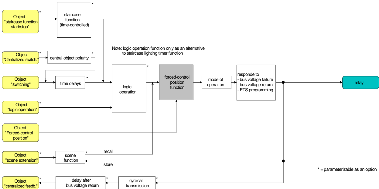
Fig. 18: Functional diagram of the forced-control position function
