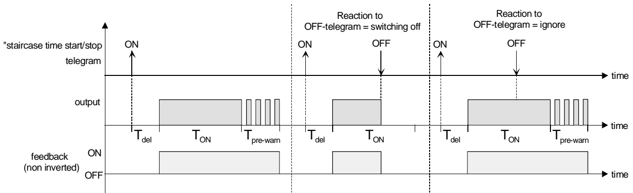
Fig. 12: Switch-off behaviour of the staircase function
